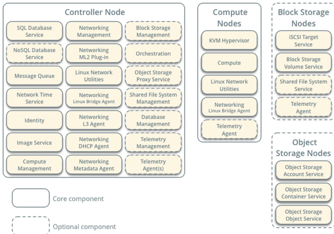
Service Layout
