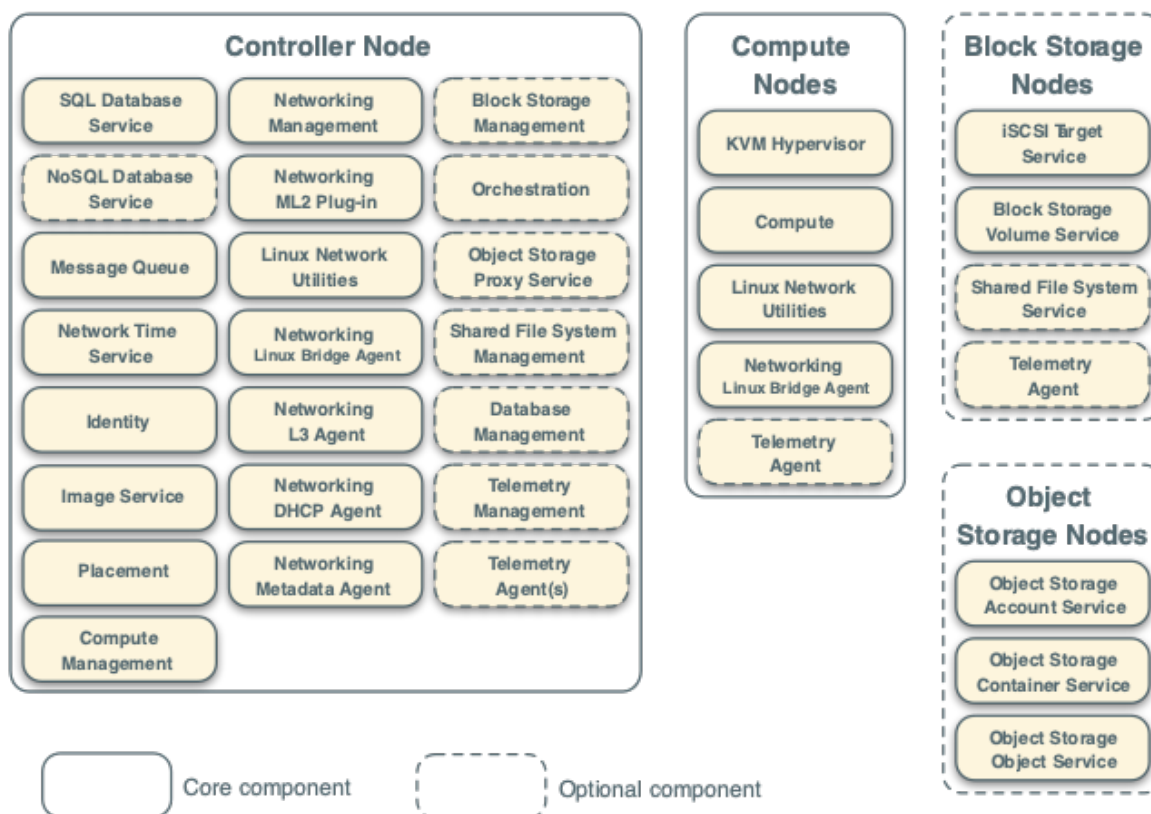
Networking Option 2: Self-Service Networks Service Layout
