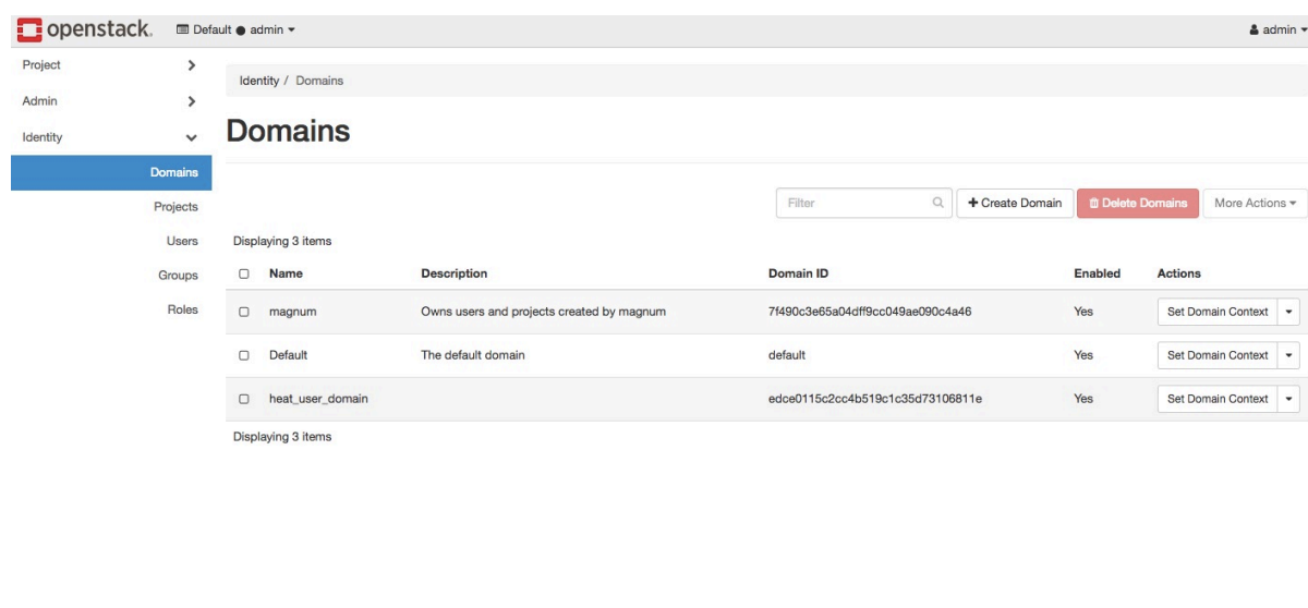
Fig. 3: Figure:Identity tab
